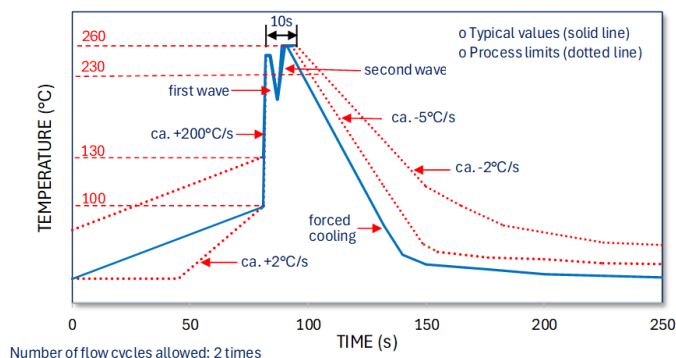
Wave Soldering Profile
