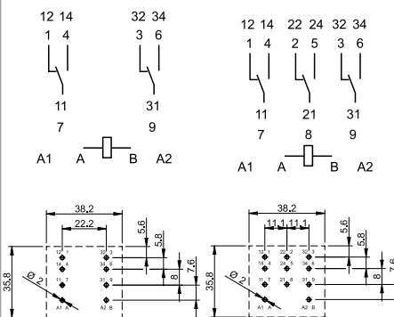
62.22 Copper side view
