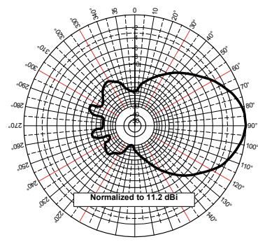
Azimuthal Pattern (X, Y or E-Plane) Representation Pattern
