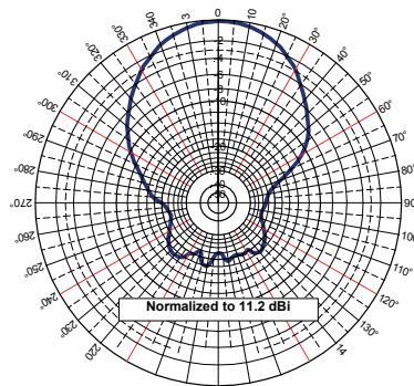
Elevation Pattern (Y, Z or H-Plane) Representation Pattern
