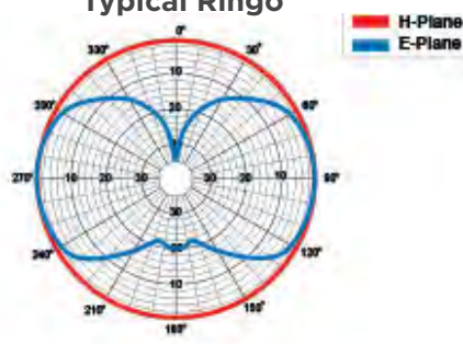
Typical Ringo
