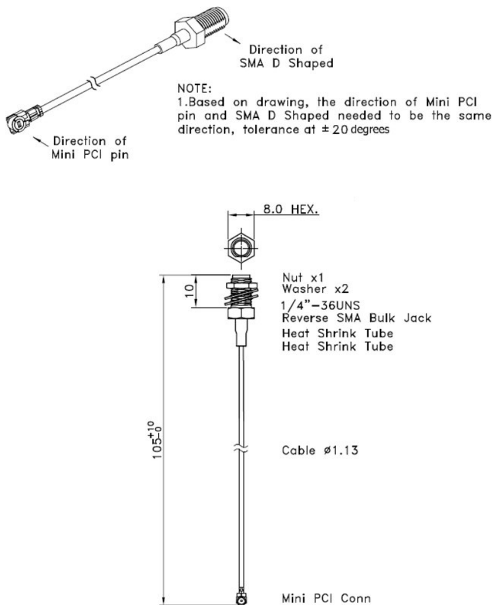
Figure 1 Physical Dimensions
