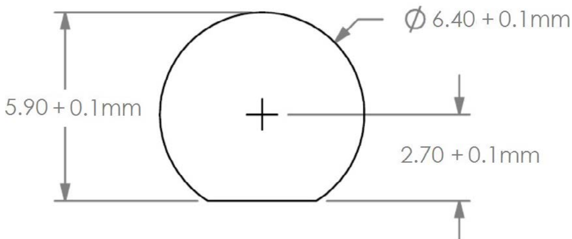
Figure 2 Recommend Cutout
