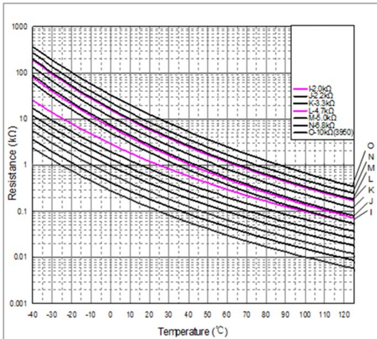
Resistance vs. Temperature
