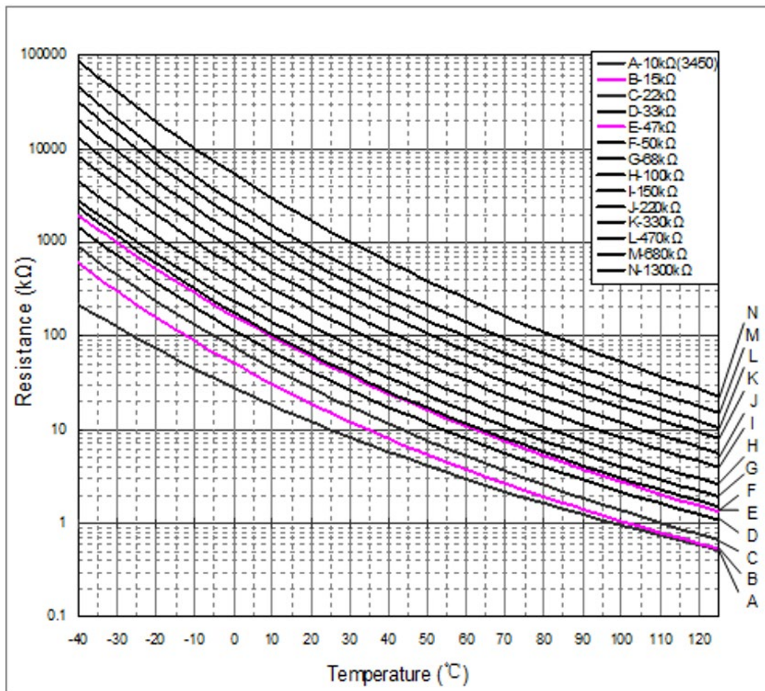
Resistance vs. Temperature
