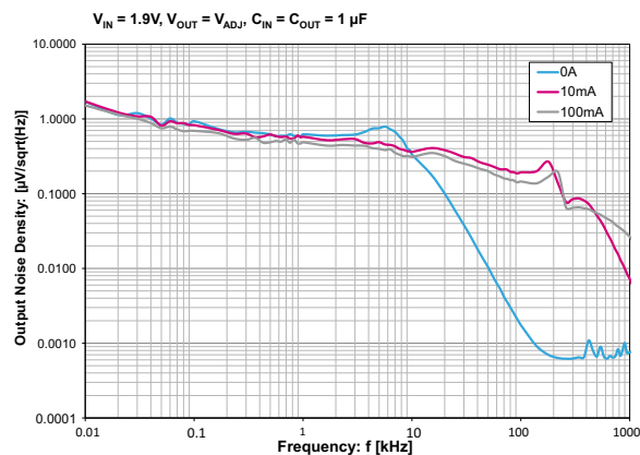
Figure 23. Output noise vs. frequency ( V_O = V_{ADJ} )
