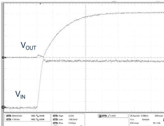
Figure 30. Startup transient
