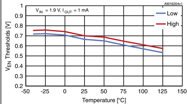
Figure 13. Enable pin thresholds vs. temp. ( V_{IN} = 1.9 V)
