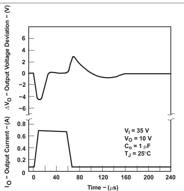
Figure 24. Load Transient Response
