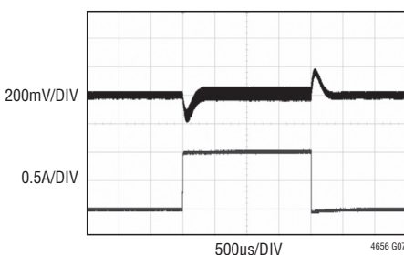
12V to 24V Boost Load Step
