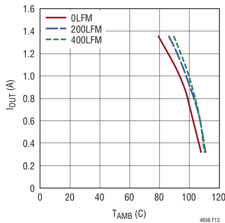
Figure 13. LTM4656 5V_{IN} , 24V_{OUT} , 500kHz, No Heat Sink
