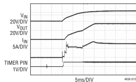
24V to 36V Boost HOT Plugged Start-Up Into 5A Load
