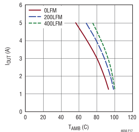
Figure 17. LTM4656 24V_{IN} , 36V_{OUT} , 650kHz, No Heat Sink
