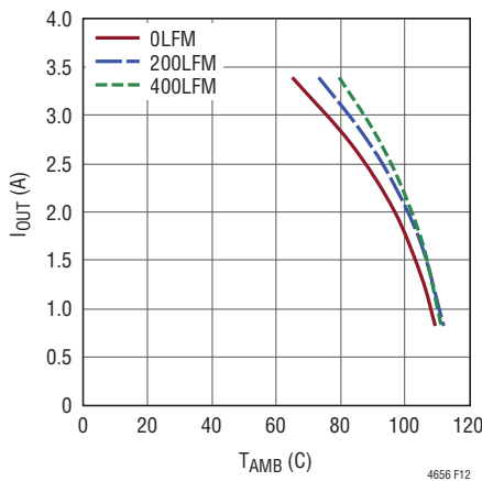
Figure 12. LTM4656 5V_{IN} , 12V_{OUT} , 400kHz, No Heat Sink
