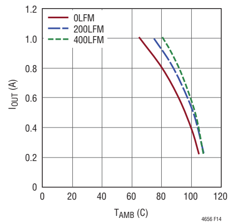
Figure 14. LTM4656 5V_{IN} , 36V_{OUT} , 500kHz, No Heat Sink
