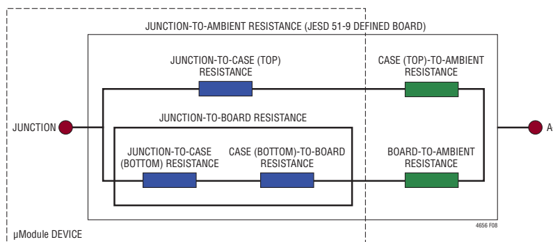
Figure 8. Graphical Representation of JESD51-12 Thermal Coefficients
