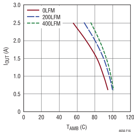
Figure 16. LTM4656 12V_{IN} , 36V_{OUT} , 650kHz, No Heat Sink
