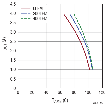
Figure 15. LTM4656 12V_{IN} , 24V_{OUT} , 550kHz, No Heat Sink
