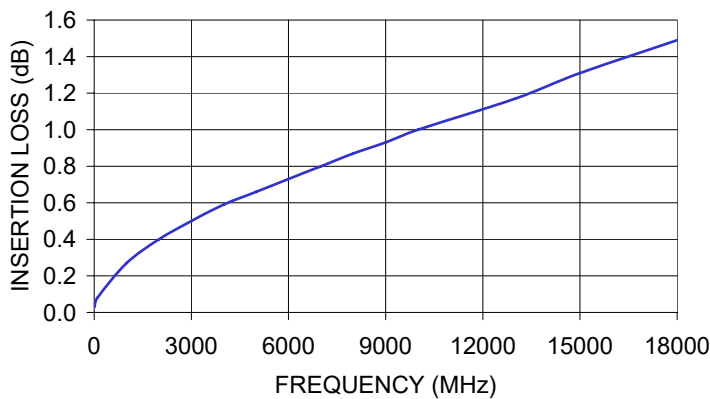
CBL-2FT-SMNM+ INSERTION LOSS
