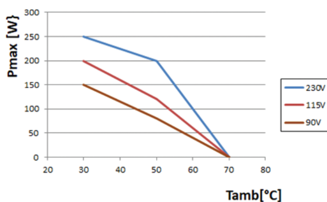
Convection only
