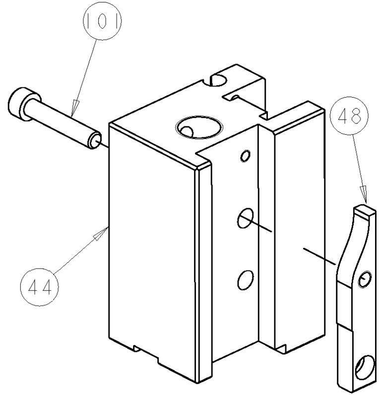
PRE-FEED 1-5/8 STROKE
