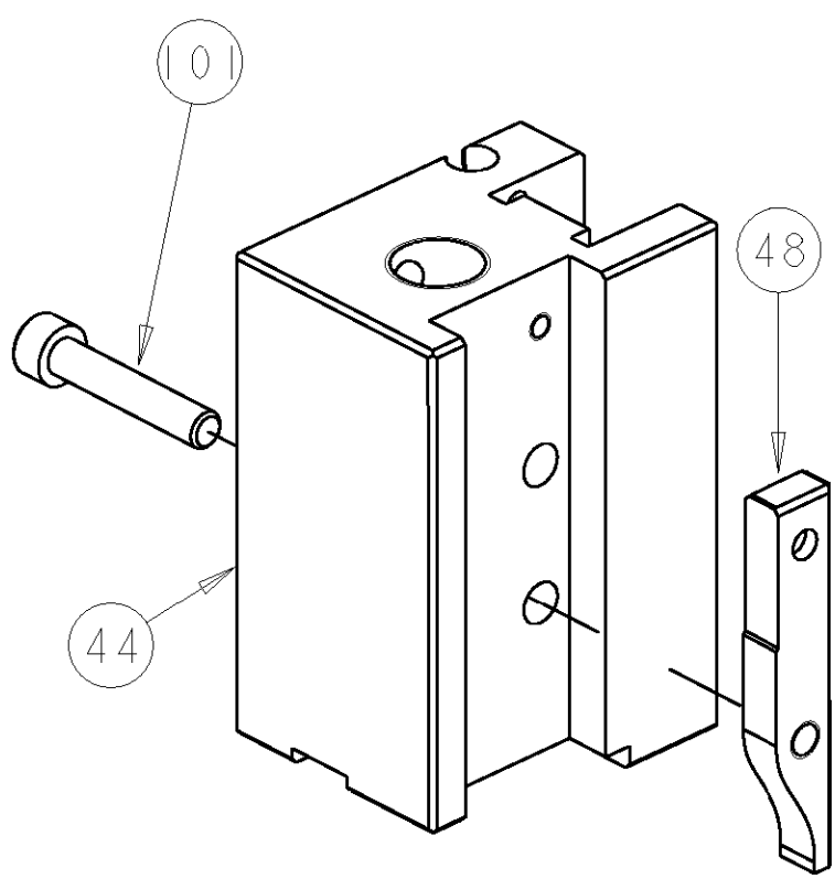
POST-FEED 1-5/8 STROKE
