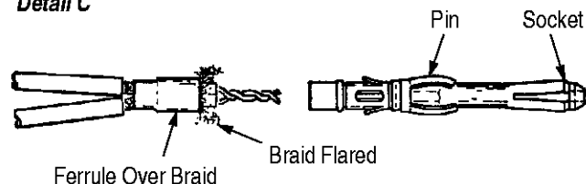
Detail C
