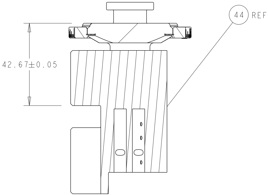
RAM SET-UP
