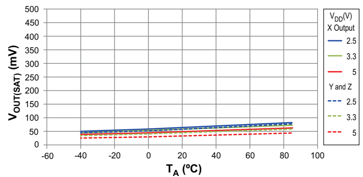
Average Low Output Voltage vs. Ambient Temperature I_{OUT} = 20\text{ mA}
