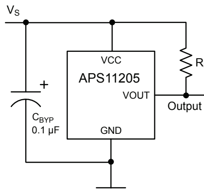
Figure 3: Typical Application Circuit
