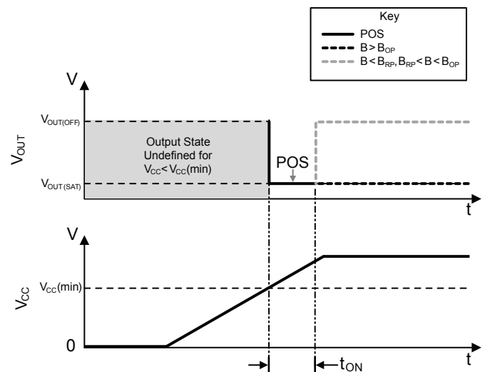
Figure 2: Power-On Sequence and Timing
