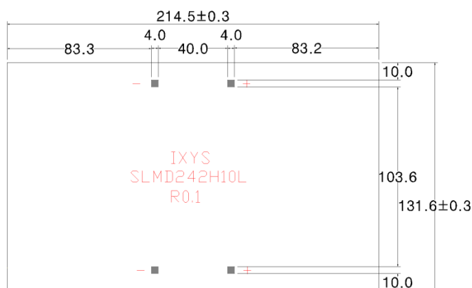
Back-side View
