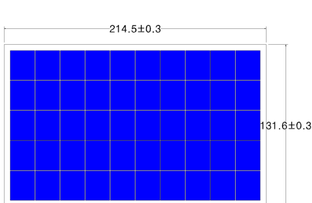
Front-side View
