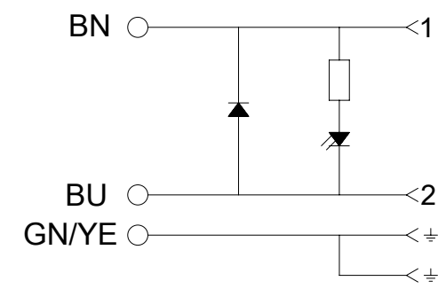
ELECTRICAL DIAGRAM C3
