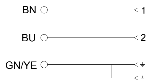
ELECTRICAL DIAGRAM 00
