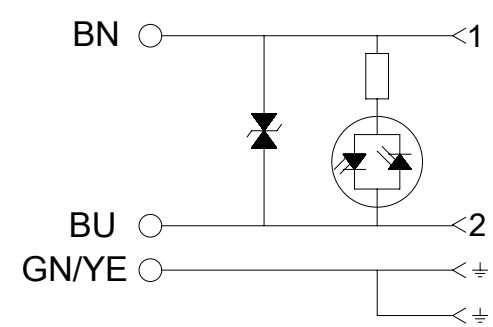
ELECTRICAL DIAGRAM S0
