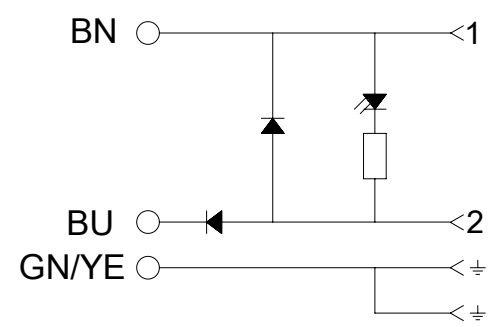
ELECTRICAL DIAGRAM C7
