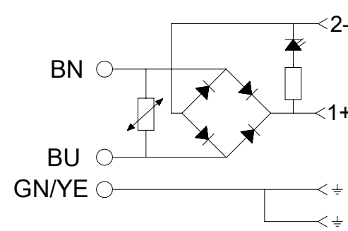
ELECTRICAL DIAGRAM R2
