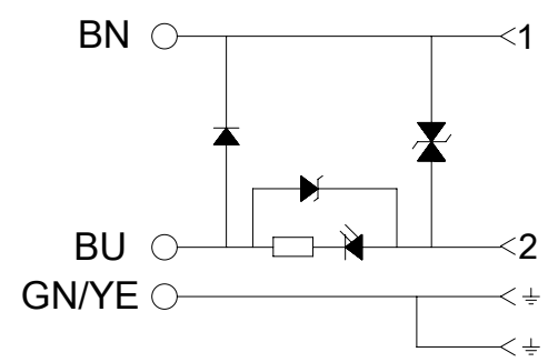
ELECTRICAL DIAGRAM NS
