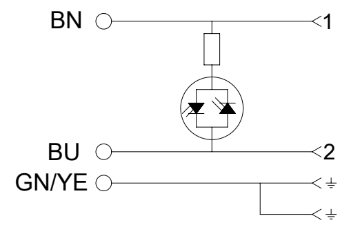
ELECTRICAL DIAGRAM A1
