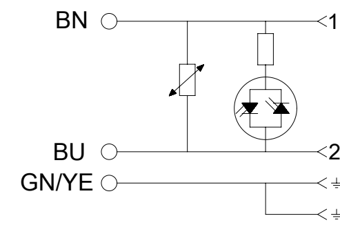
ELECTRICAL DIAGRAM C4
