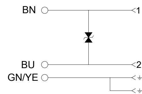
ELECTRICAL DIAGRAM S1
