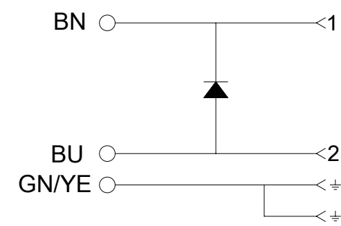
ELECTRICAL DIAGRAM E0
