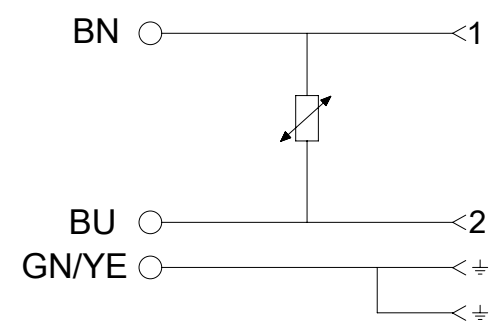
ELECTRICAL DIAGRAM D0
