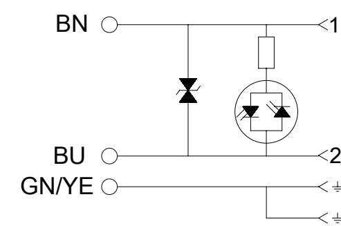
ELECTRICAL DIAGRAM S3
