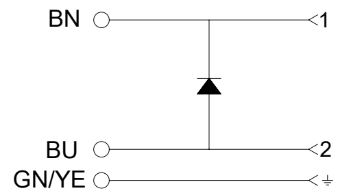
ELECTRICAL DIAGRAM E0
