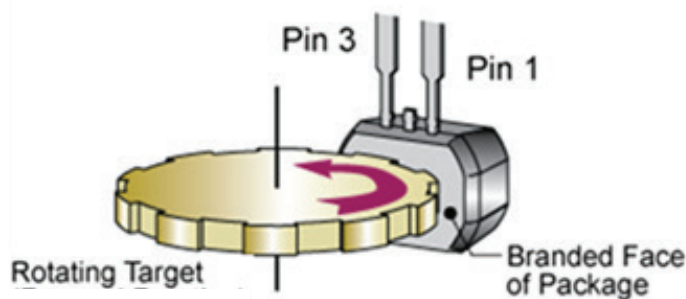
Figure 6: Left-to-Right, Pin 1 to Pin 3 Direction of Target Rotation.
