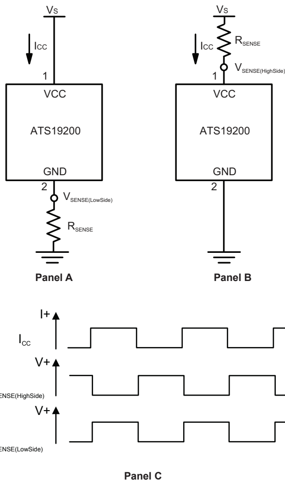
Figure 7: Alternative Polarity Configurations Using Two-Wire Sensing.
