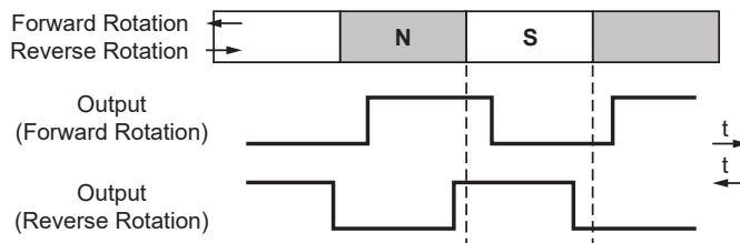
Figure 8a: Output Protocol (-FOOOOxx Variants)
