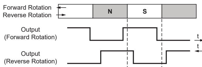
Figure 8b: Output Protocol (-ROOOOxx Variants)
