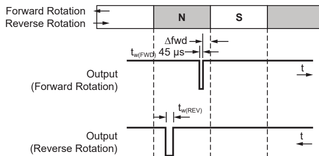
Figure 10: Output Protocol (-FSxxCxx Variants)
