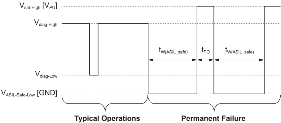
Figure 20: ASIL Output Behavior (-xxxxxEx-A Variants)
