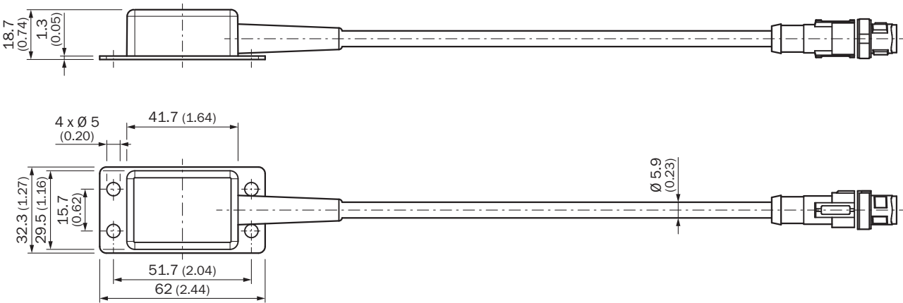
Dimensions in mm (inch)
