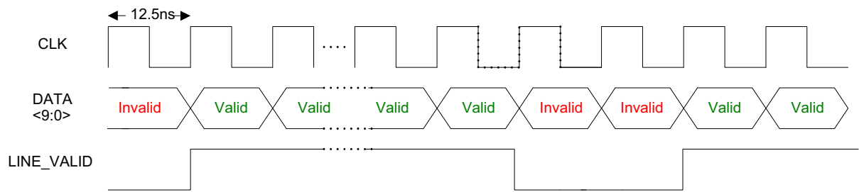
Figure 20. LINE_VALID Timing
