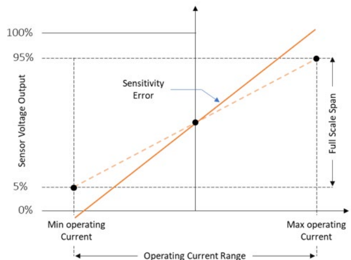
Figure 20: Exaggerated Gain Error
