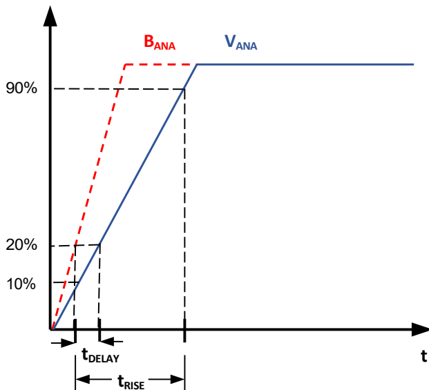
Figure 15: CT220 Propagation Delay and Rise Time Curve
