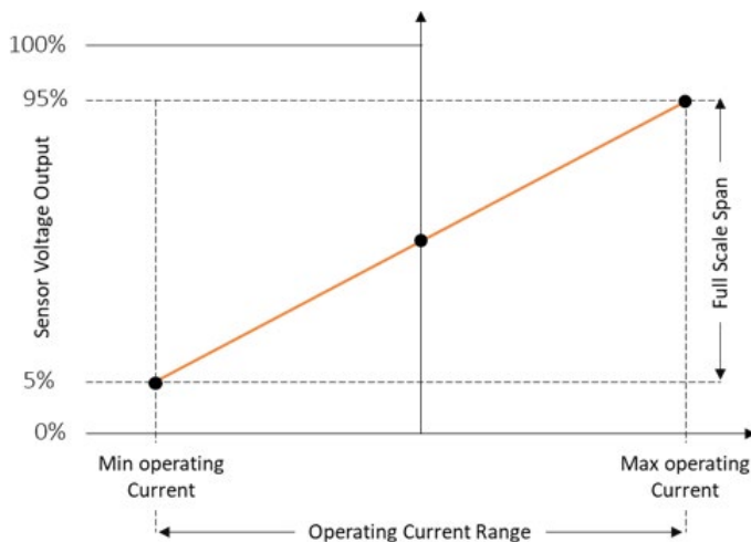
Figure 18: Ideal Transfer Line
