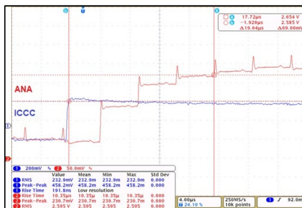
Figure 8: Response Time for CT220
