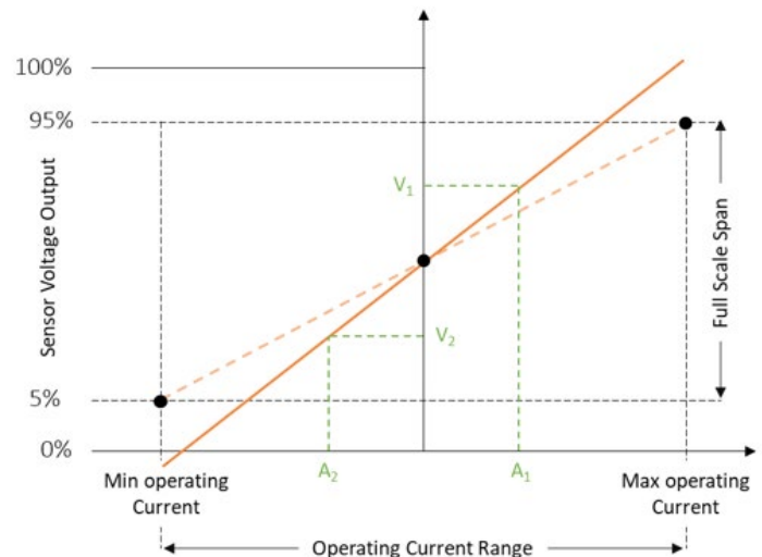
Figure 23: Gain Calibration
