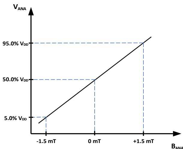
Figure 13: Linear Output Voltage Range vs. Measured Current for G = 300 mV/V/mT and current range of +1.5 mT.
