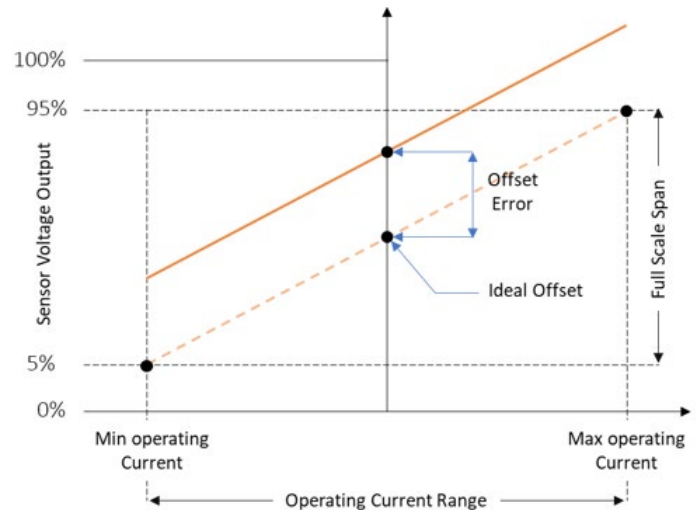
Figure 19: Exaggerated Offset Error
