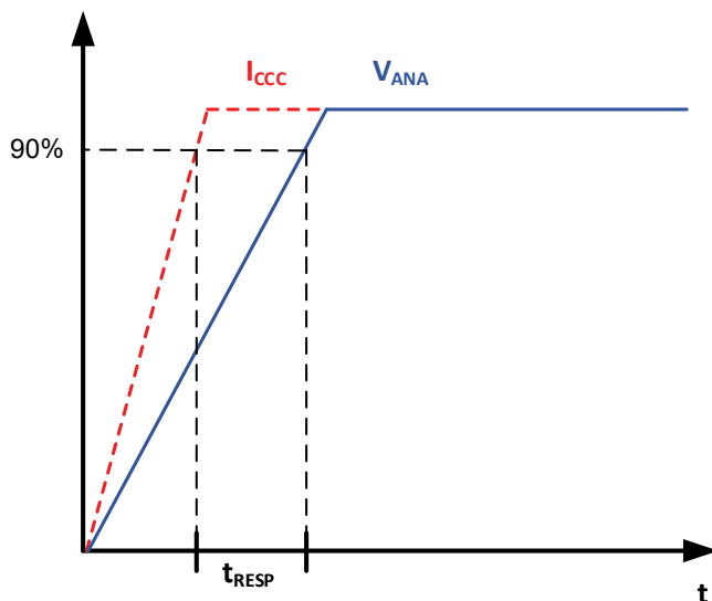
Figure 16: CT220 Response Time Curve
