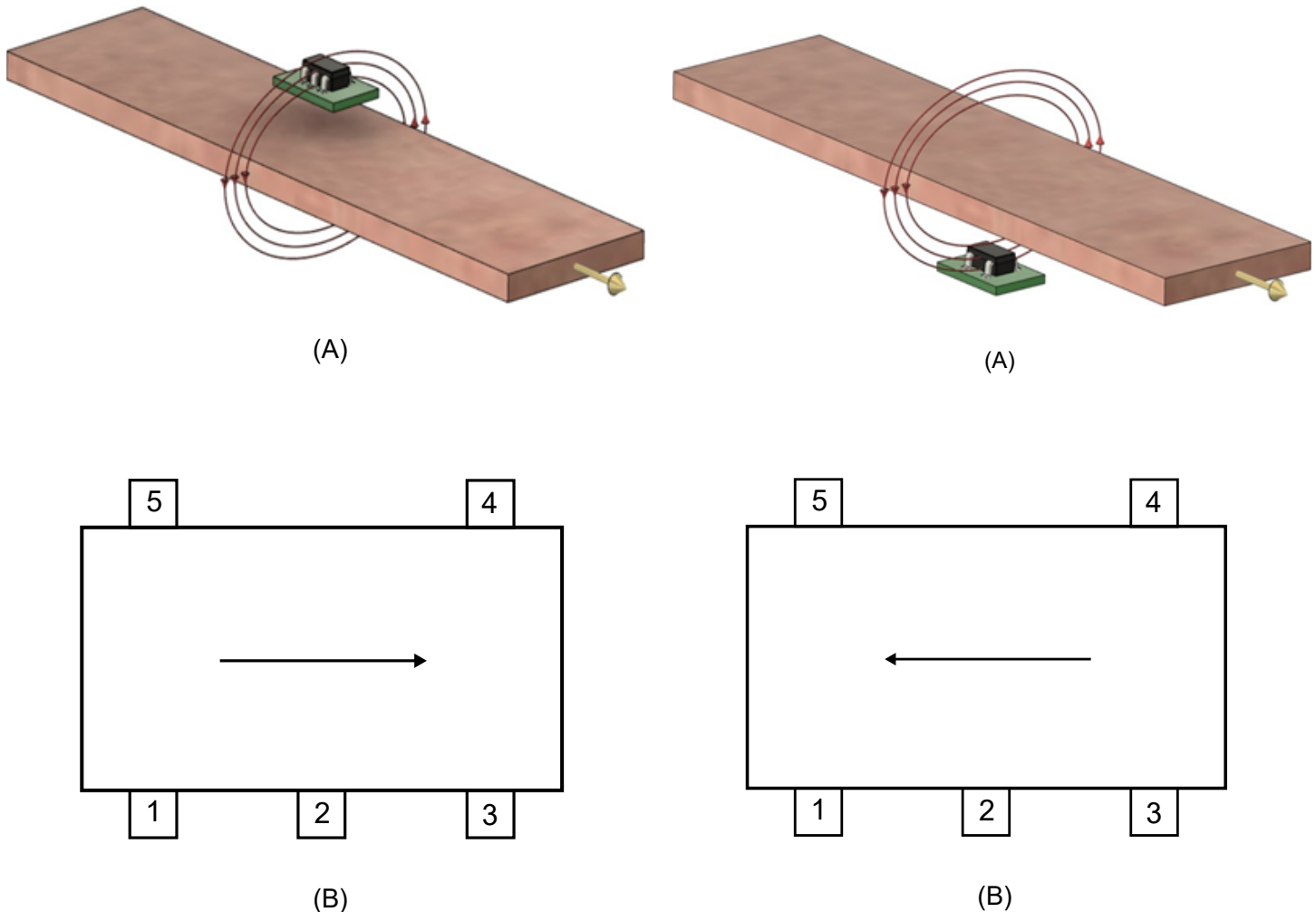
Figure 25: CT220 measuring unipolar current in a busbar below it where (A) indicates the unipolar current and magnetic field directions, and (B) is the direction of unipolar current flow that the CT220 must be oriented.
