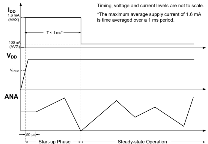
Figure 17: CT220 Power-On Timing Diagram
