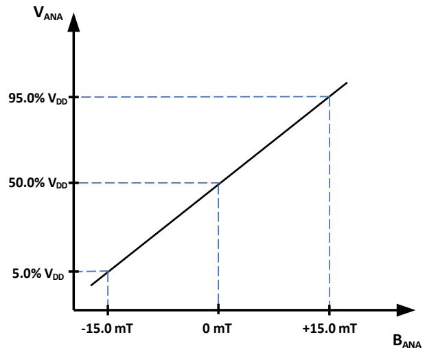
Figure 14: Linear Output Voltage Range vs. Measured Current for G = 30 mV/V/mT and current range of +15.0 mT.
