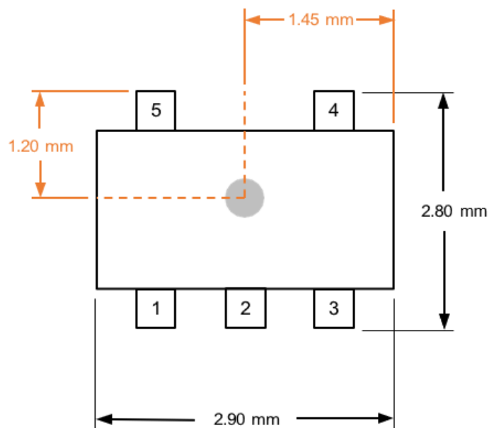
Figure 27: XtremeSense TMR Sensor Location in X and Y Dimensions for CT220 in SOT23-5 Package
