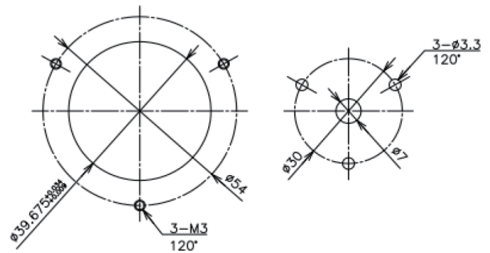
Servo Mount
