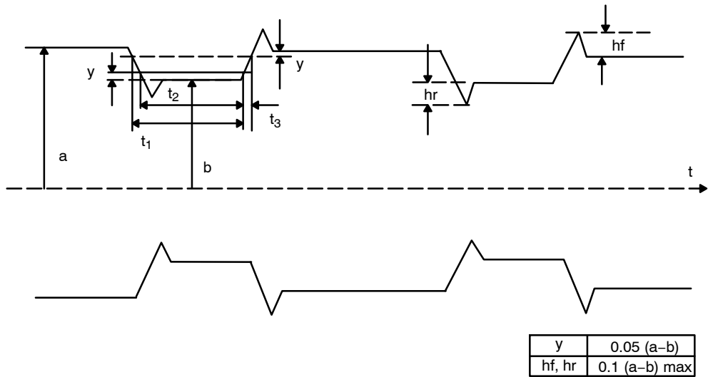
Figure 3. 10% Modulation Waveform
