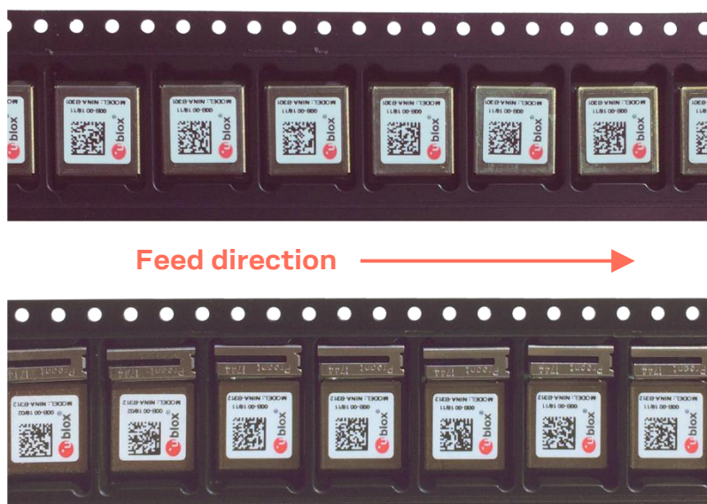
Figure 17: Orientation of NINA-B3 modules on tape
