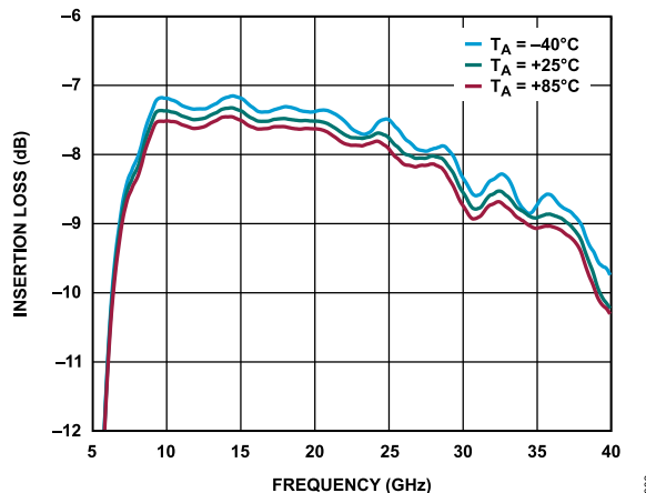
Figure 8. Insertion Loss P1 vs. Frequency over Temperature
