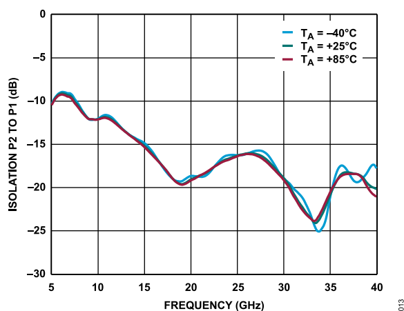
Figure 13. Isolation P2 to P1 vs. Frequency over Temperature
