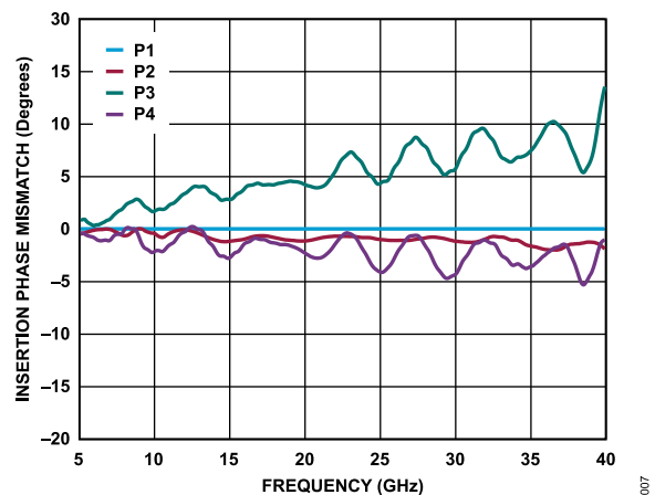
Figure 7. Insertion Phase Mismatch vs. Frequency, All Paths Normalized to P1
