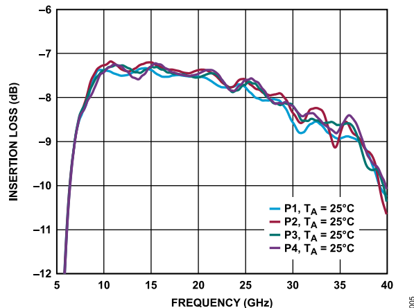
Figure 5. Insertion Loss vs. Frequency
