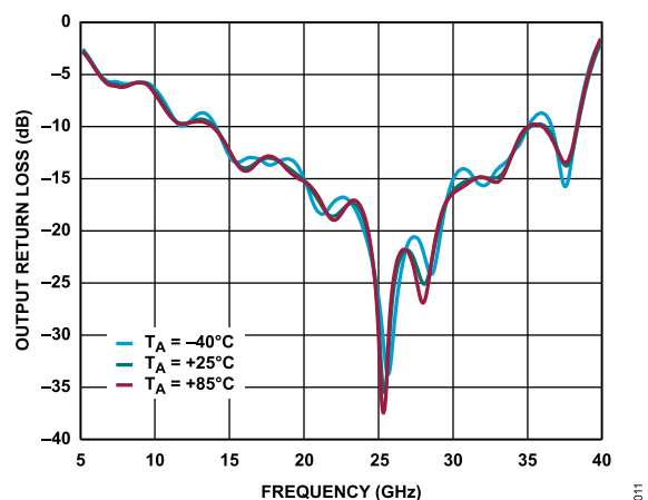
Figure 11. Output Return Loss P1 vs. Frequency over Temperature
