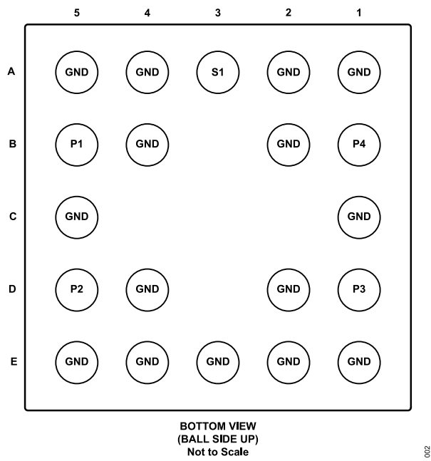
Figure 2. Pin Configuration (Bottom View)
