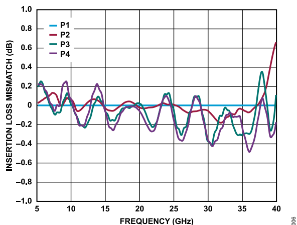
Figure 6. Insertion Loss Mismatch vs. Frequency, All Paths Normalized to P1
