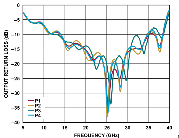
Figure 10. Output Return Loss vs. Frequency (P1, P2, P3, and P4)
