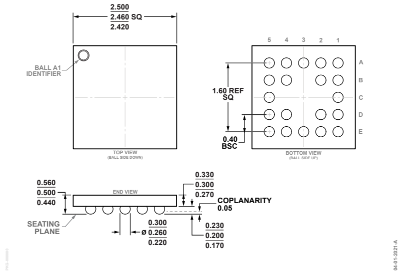
Figure 15. 20-Ball Wafer Level Chip Scale Package [WLCSP] (CB-20-17) Dimensions shown in millimeters
