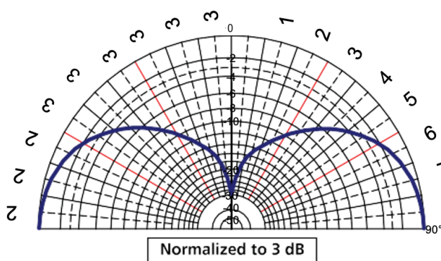
Elevation Pattern (Y, Z, or H-plane)
