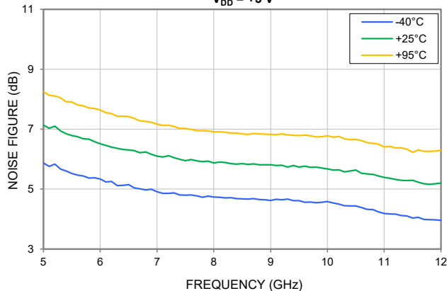
NOISE FIGURE vs. TEMPERATURE V_{DD} = +5 \text{ V}
