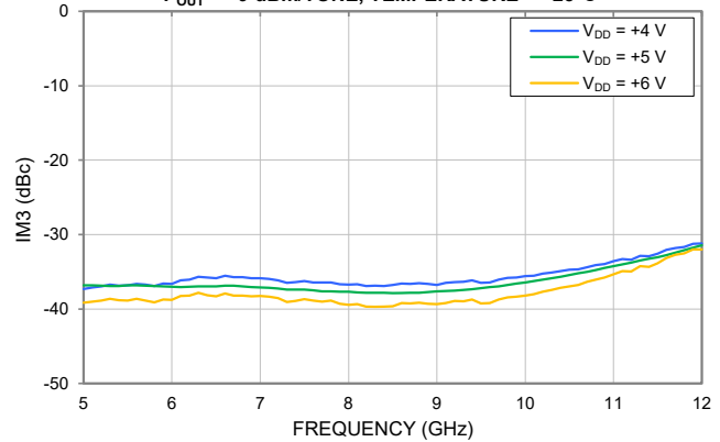
IM3 vs. DEVICE VOLTAGE P_{OUT} = +9 \text{ dBm/TONE} , TEMPERATURE = +25°C
