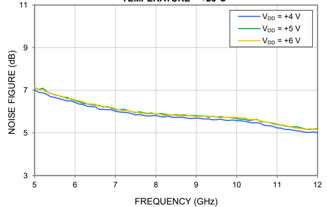
NOISE FIGURE vs. DEVICE VOLTAGE TEMPERATURE = +25°C
