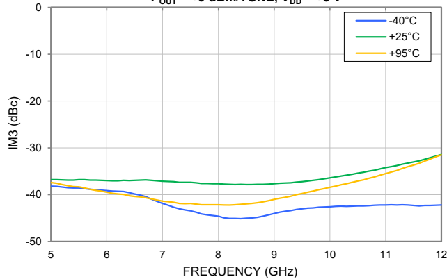
IM3 vs. TEMPERATURE P_{OUT} = +9 \text{ dBm/TONE} , V_{DD} = +5 \text{ V}
