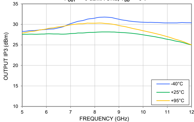
OUTPUT IP3 vs. TEMPERATURE P_{OUT} = +9 \text{ dBm/TONE} , V_{DD} = +5 \text{ V}
