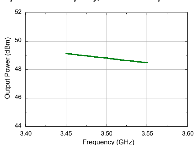
Output Power vs. Frequency, 2.5dB Gain Compression
