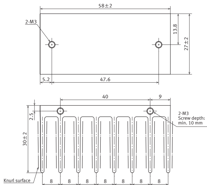
External dimensions
