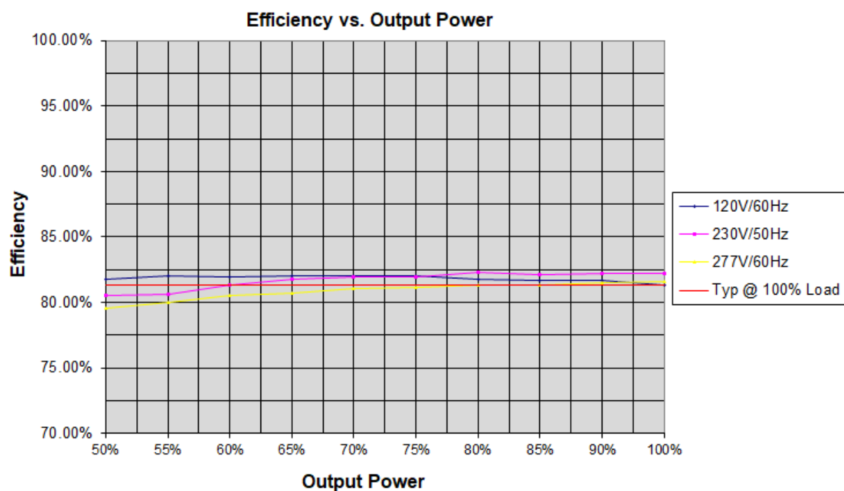
Efficiency Curve (Typical)
