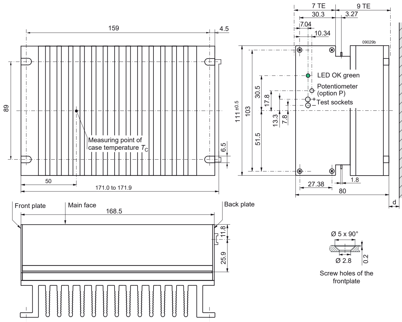
Fig. 14 Case K01 for PSK models, weight 1.6 kg Aluminum, fully enclosed, black finish EP powder-coated, and self cooling.
