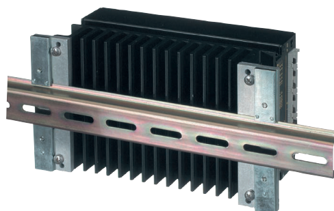
Fig. 20 DIN-rail mounting assembly HZZ0615-G
