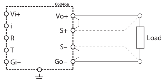
Fig. 9 Sense lines connection
