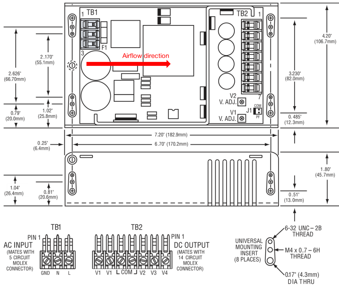
Figure 1. Mechanical Drawing
