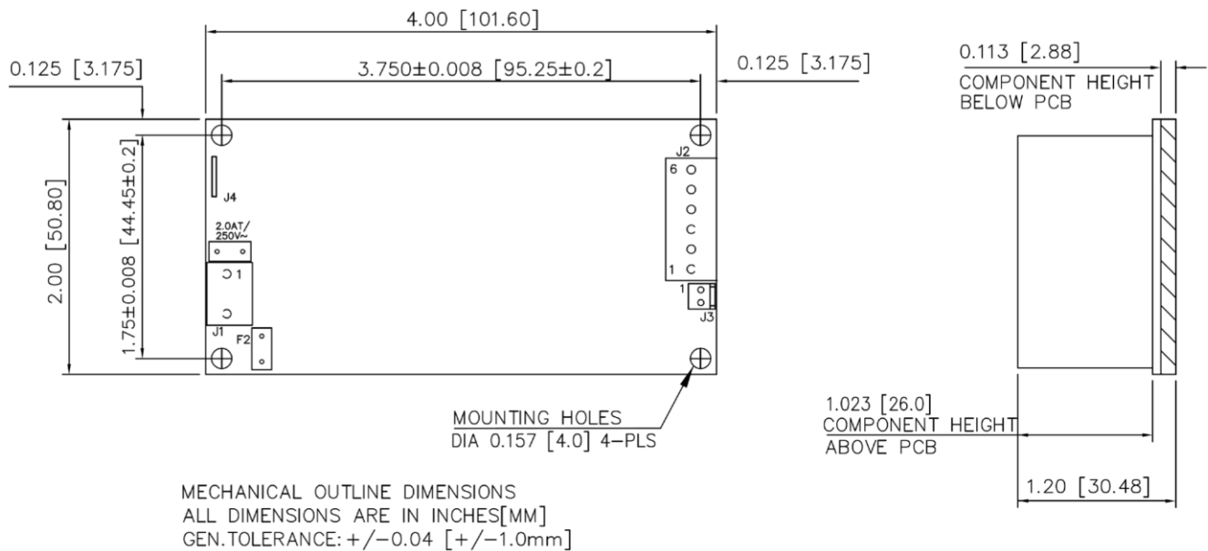
Figure 4. Mechanical Drawing MBC60-3xxxG
