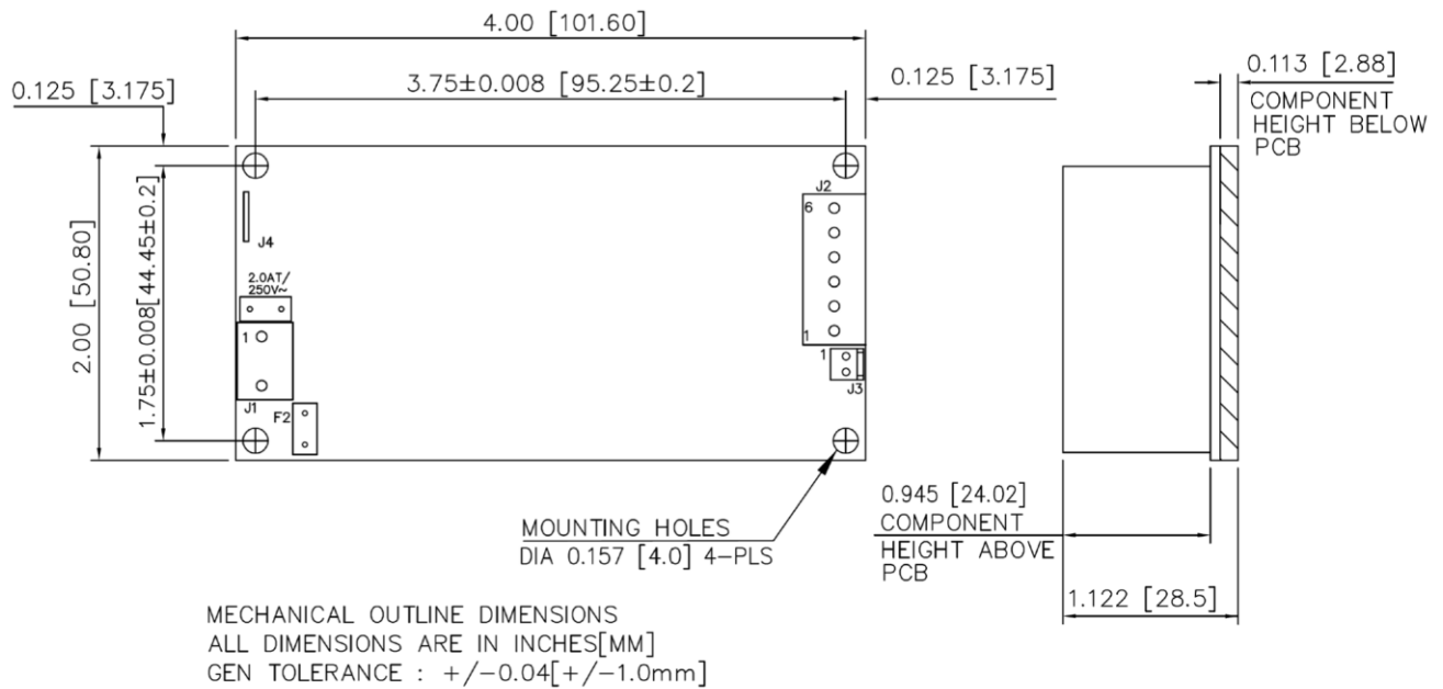
Figure 3. Mechanical Drawing MBC60-1xxxG
