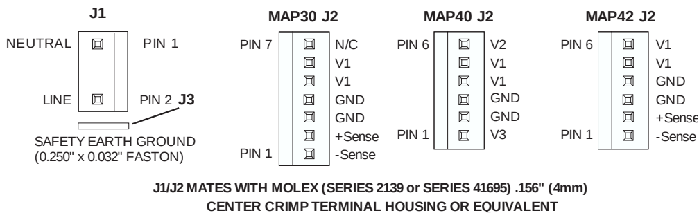
Figure 4. Electrical Connectors
