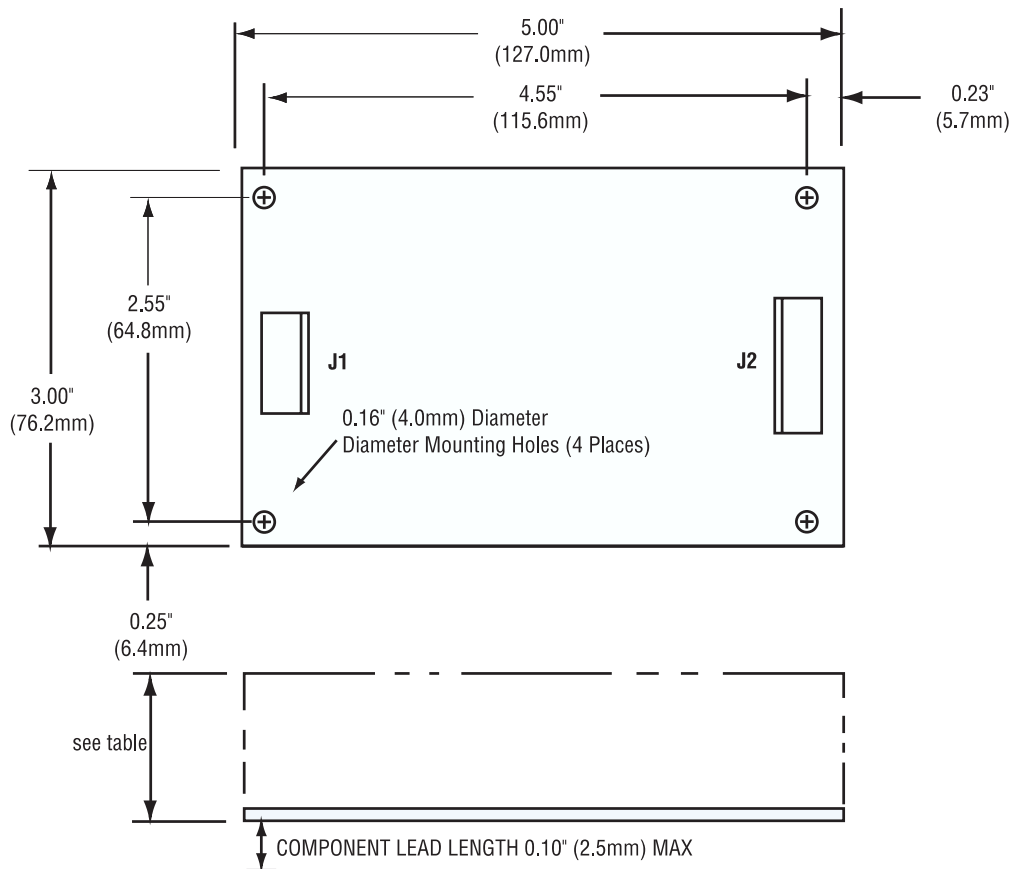
Figure 5. Mechanical Drawing
