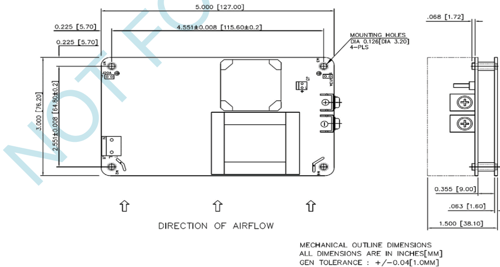
Figure 1. Mechanical Drawing
