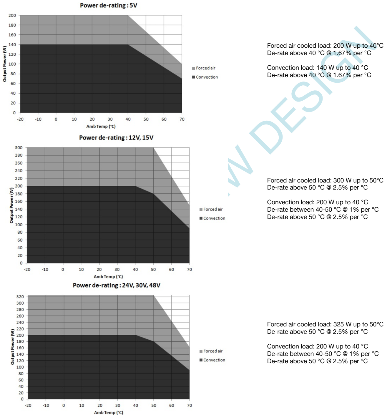
Figure 1. Derating Curves
