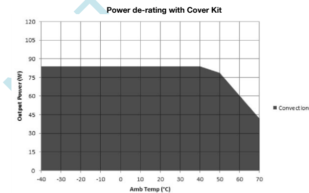
Figure 1. Derating Curves
