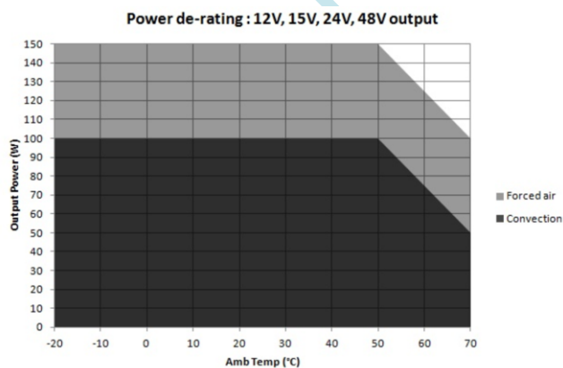
Figure 1. Derating Curves
