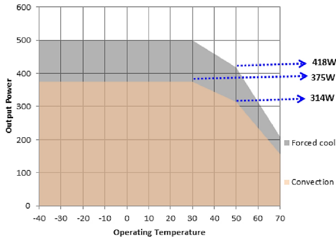
Figure 9. Power Derating Curve 15 V
