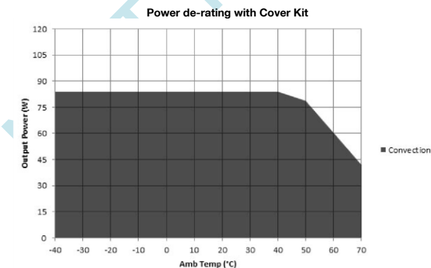
Figure 1. Derating Curves
