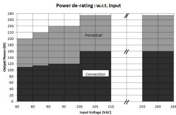
Figure1. Derating Curves
