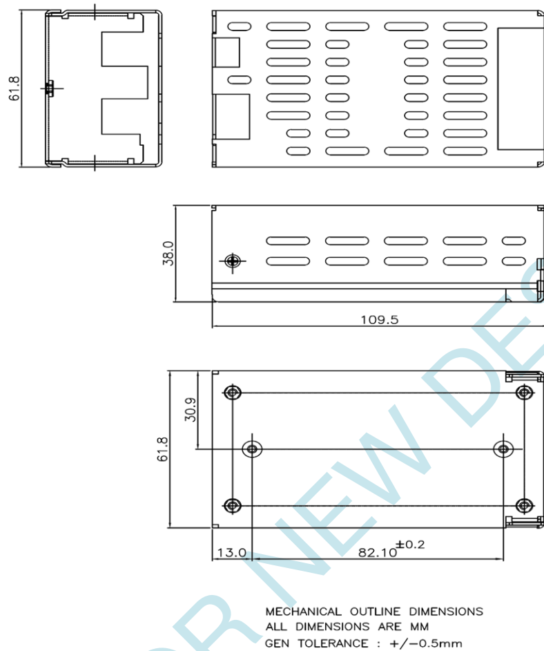
Figure 4. Mechanical Drawing with Cover Kit
