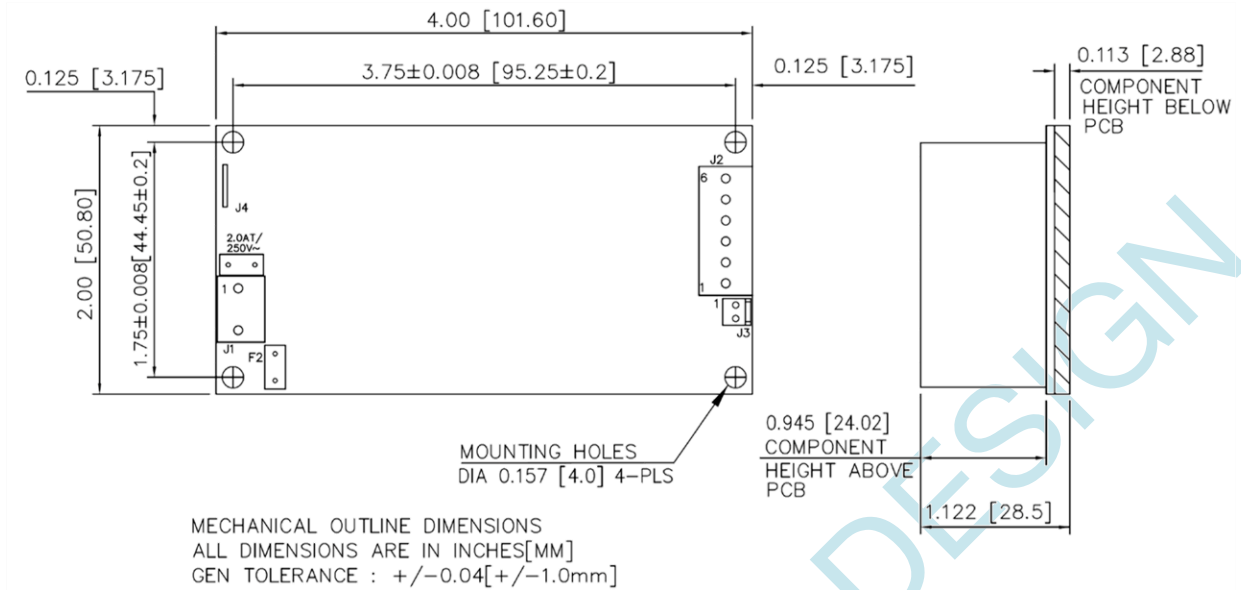
Figure 2. Mechanical Drawing ABC40-1xxxG
