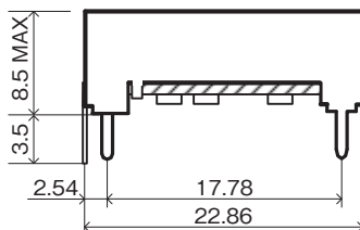
Side surface
