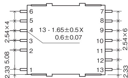
Rear surface
