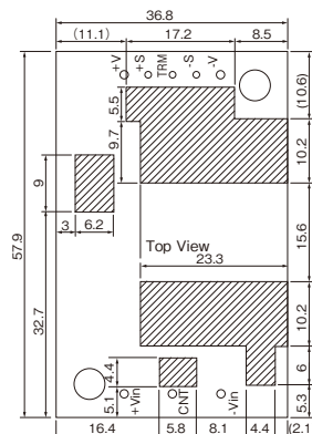
Fig.2-1 Prohibition area of wiring pattern
