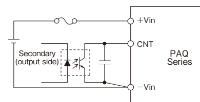
Fig.10-1 CNT connection
