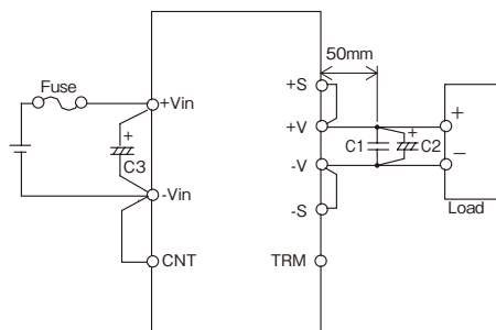
Fig.1-2 Basic Connection
