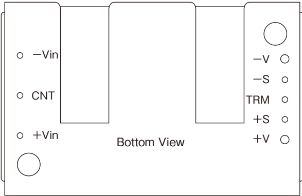
Input and Outoput Terminal Configurations (Bottom View)
