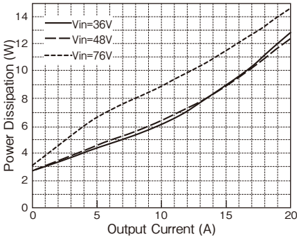
Fig.1-8 PAQ100S48-5/B Power dissipation vs Output Current (Output voltage: Nominal, Ta=60°C; typical value)
