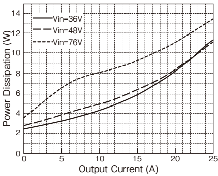
Fig.1-7 PAQ100S48-3R3/B Power dissipation vs Output Current (Output voltage: Nominal, Ta=60°C; typical value)
