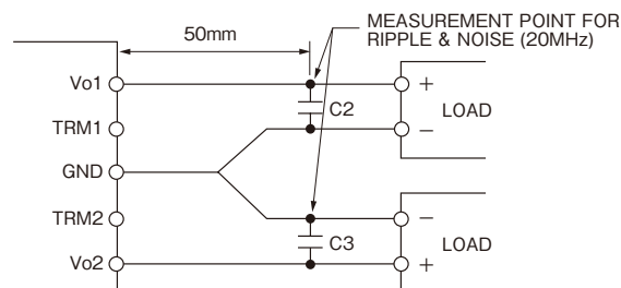
Fig.4-1: Measurement method for ripple and noise
