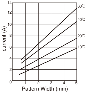
Fig.2-2 Characteristic of current allowance
