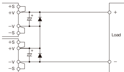
Fig.12-1 Series Operation for High Output Voltage Application
