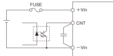
Fig.10-1 : CNT connection
