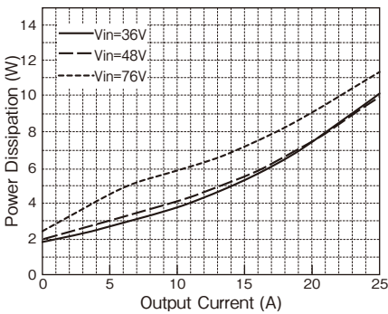
Fig.1-6 PAQ100S48-2R5/B Power dissipation vs Output Current (Output voltage: Nominal, Ta=60°C; typical value)
