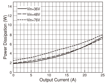
Fig.1-5 PAQ100S48-1R8/B Power dissipation vs Output Current (Output voltage: Nominal, Ta=60°C; typical value)
