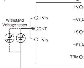
1.5kVDC 1minute (10mA) Fig.19-1 Withstand Voltage Test for Input-Output
