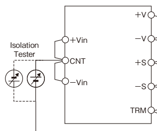
Fig.20-1 Isolation test
