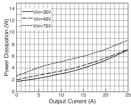
Fig.1-4 PAQ100S48-1R2/B Power dissipation vs Output Current (Output voltage: Nominal, Ta=60°C; typical value)
