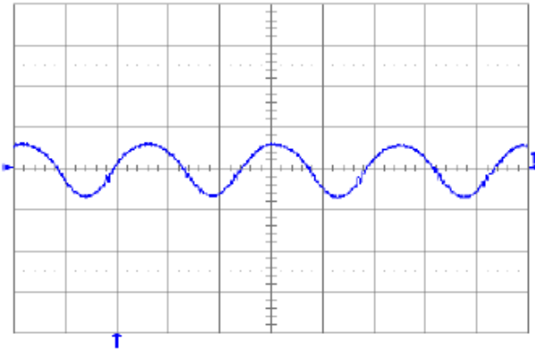
Fig. 8.0V.11: Output voltage ripple (50 mV/div.) at full rated load current into a resistive load with C_o = 10\mu F tantalum + 1\mu F ceramic and V_{in} = 48V . Time scale: 1 \mu s/div.
