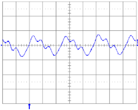
Fig.3.3V.13: Output voltage ripple (20 mV/div.) at full rated load current into a resistive load with C_o = 10\mu\text{F} tantalum + 1\mu\text{F} ceramic and V_{in} = 48\text{V} . Time scale: 1\mu\text{s}/\text{div} .
