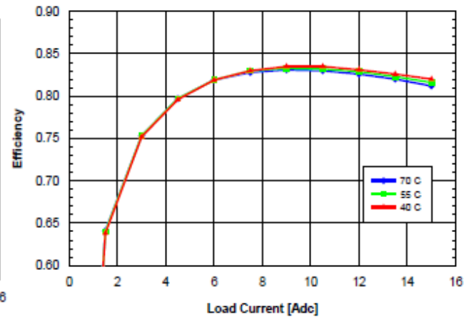
Fig. 1.2V.6: Efficiency vs. load current and ambient temperature for SQ48T/S15012 converter mounted vertically with V_{in} = 48\text{V} and air flowing from pin 3 to pin 1 at a rate of 200LFM (1.0 m/s).
