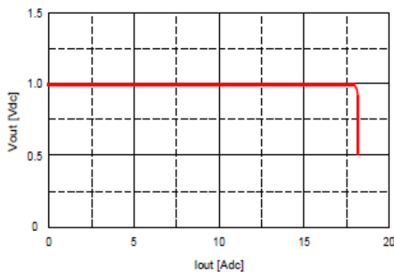
Fig. 1.0V.17: Output voltage vs. load current showing current limit point and converter shutdown point. Input voltage has almost no effect on current limit characteristic.
