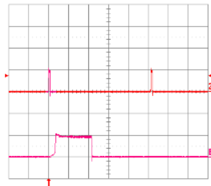
Fig. 3.3V.18: Load current (top trace, 10\text{A}/\text{div.} , 20\text{ ms}/\text{div.} ) into a 10\text{ m}\Omega short circuit during restart, at V_{in} = 48\text{V} . Bottom trace ( 20\text{A}/\text{div.} , 1\text{ms}/\text{div.} ) is an expansion of the on-time portion of the top trace.
