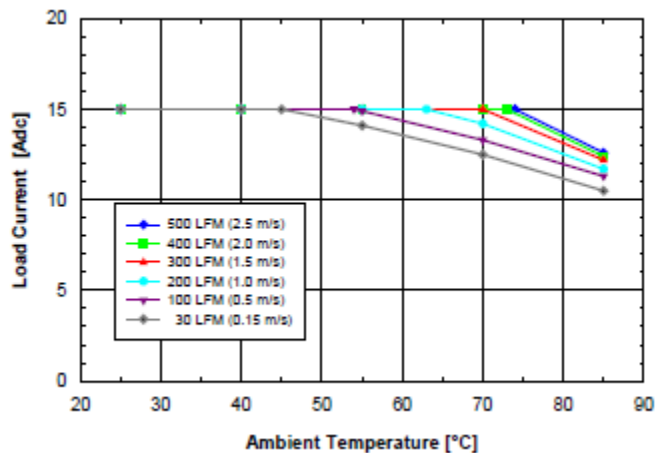
Figure 3.3V.4 Available load current vs. ambient air temperature and airflow rates for SQ48S15033 converter with D height pins mounted horizontally with V_{in} = 48V , air flowing from pin 3 to pin 1, and maximum FET temperature \leq 120^{\circ}C .
