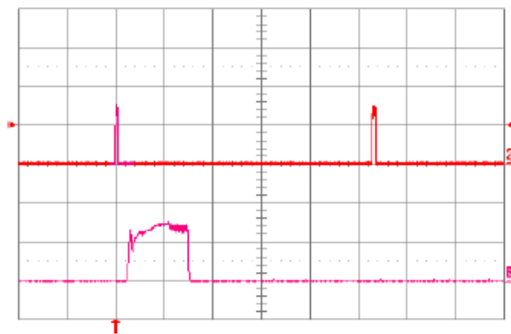
Fig. 8.0V.16: Load current (top trace, 5A/div., 20 ms/div.) into a 10 m\Omega short circuit during restart, at V_{in} = 48V . Bottom trace (5A/div., 1ms/div.) is an expansion of the on-time portion of the top trace.
