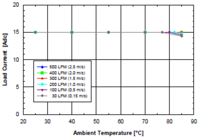
Figure 1.2V.4 Available load current vs. ambient air temperature and airflow rates for SQ48S15012 converter with D height pins mounted horizontally with V_{in} = 48V , air flowing from pin 3 to pin 1, and maximum FET temperature \leq 120^{\circ}C .
