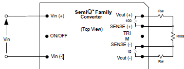
Figure 2. Remote sense circuit configuration
