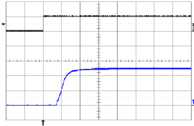
Fig. 5.0V.9: Turn-on transient at full rated load current (resistive) with no output capacitor at V_{in} = 48V , triggered via ON/OFF pin. Top trace: ON/OFF signal (5V/div.). Bottom trace: output voltage (2V/div.). Time scale: 2ms/div.
